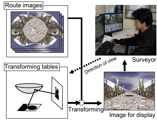
Fig. 9. Whole process flow of the simulational environment.
