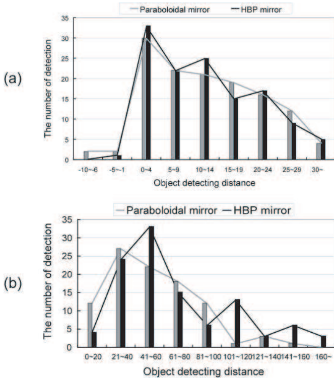
Fig. 16. Histograms of the detection distances. (a) detections of objects on the alleys. (b) detections of objects on the main route.
