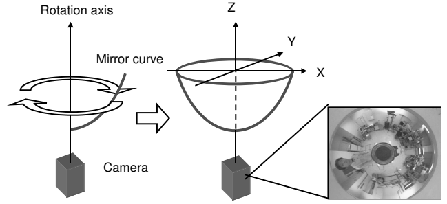
Fig. 1. An example of a conventional omnidirectional imaging system with a convex mirror. It consists of a camera and a rotational convex mirror. The optical axis of the camera is aligned to the mirror’s rotational axis.
