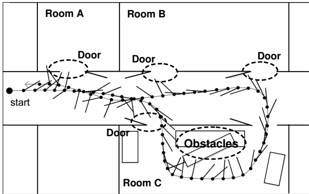
Fig. 7. Experimental scene in which the cart with the HBP mirror system drove. The scene is constructed by a passage and rooms. Doors of the room A, B and C are opened for the surveyor to be able to look in. The cart starts driving from the left edge of the figure, then goes into the room C including some obstacles and goes out to return to the starting point, described by a curve. Dots with short lines describe positions of the cart and the view direction of the surveyor at that time, respectively.
