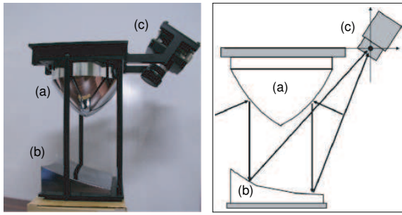
Fig. 2. Prototype of the HBP mirror system and its geometry model. A ray from a point in a scene is reflected by the HBP mirror(a) and reflected again by a parabolic mirror(b) to concentrate on a perspective camera(c).
