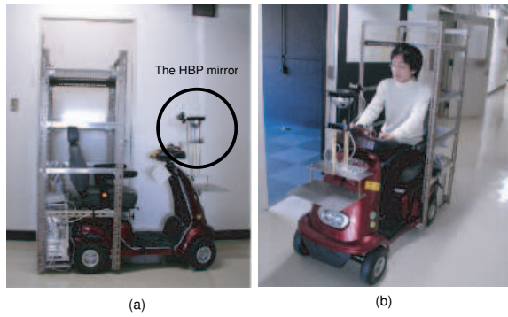
Fig. 6. The HBP mirror system mounted on an electric cart for remote surveillance. (a) overview of the cart. The HBP mirror system is fixed at the front of the steering wheel (even if a driver steers, the HBP mirror system does not rotate). (b) driving scene for surveillance.
